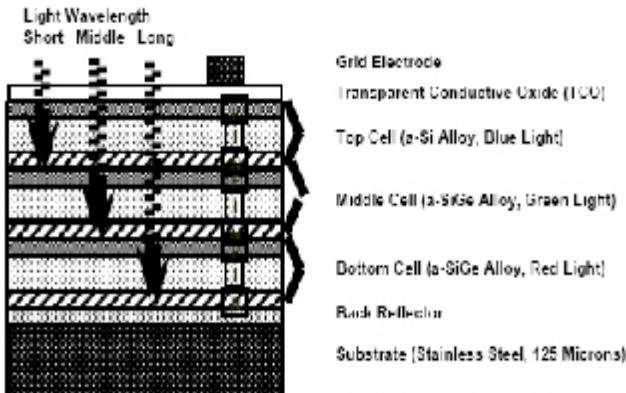
Figure 1 Uni-Solar Triple Junction Cell Light Absorption
